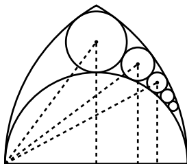
Figure 15. Arch (adapted from [21, p. 289]).
