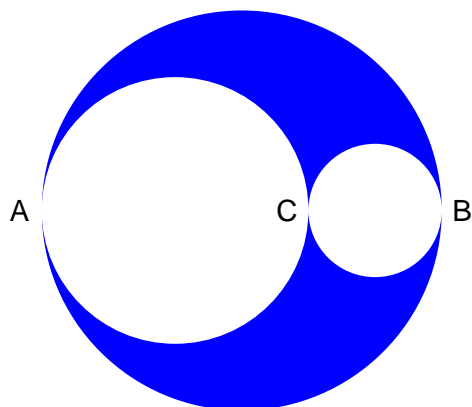
Figure 4. Proof by reflection.
