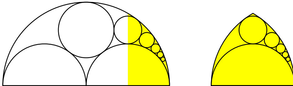
Figure 17. Reflecting the symmetric arbelos into the arch.
