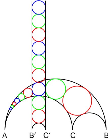
Figure 12. Inversion of Figure 10.
