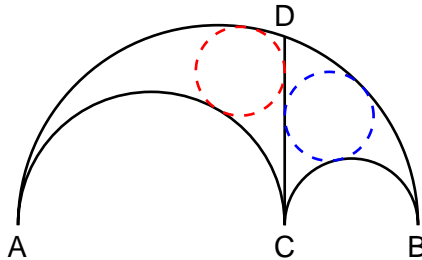
Figure 6. The twin circles.
