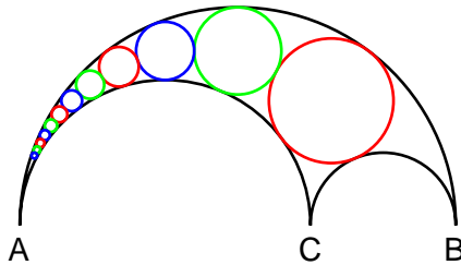
Figure 10. A classical diagram.
