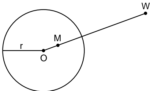
Figure 7. Reflection in a circle: (OM)(OW) = r^2 .
