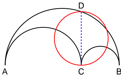
Figure 3. An area property of the arbelos.
