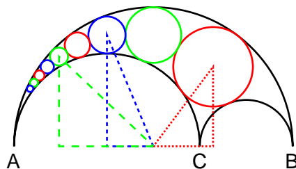
Figure 13. Some Pythagorean triangles.
