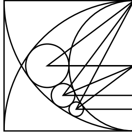
Figure 16. Pythagorean triangles (adapted from [9]).
