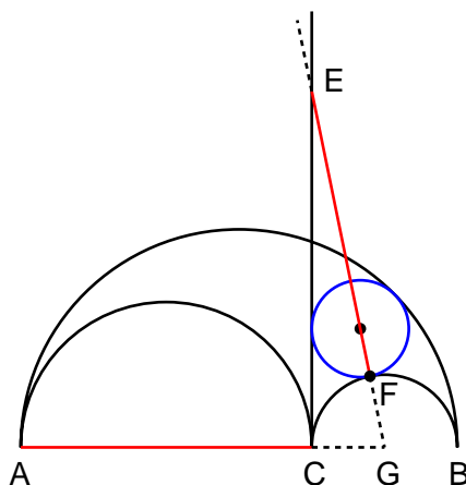
Figure 19. Corrected problem: AC = EF .
