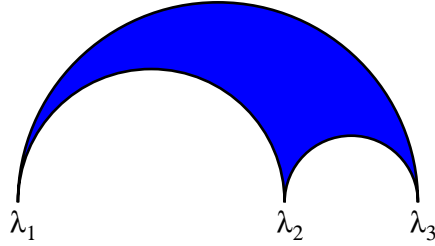
Figure 18. Eigenvalues and Mohr's arbelos.
