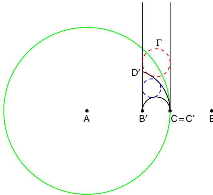
Figure 8. Inversion of Figure 6.
