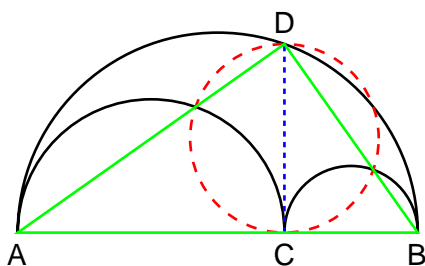
Figure 5. A mean proportional.
