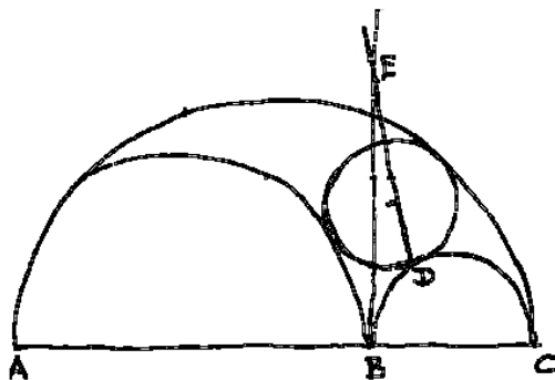
Figure 1. A correspondent’s hand-drawn puzzle.
